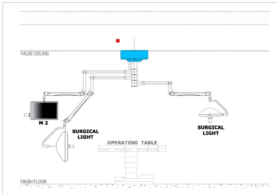
BA 1.3 ( SIDEVIEW D )
